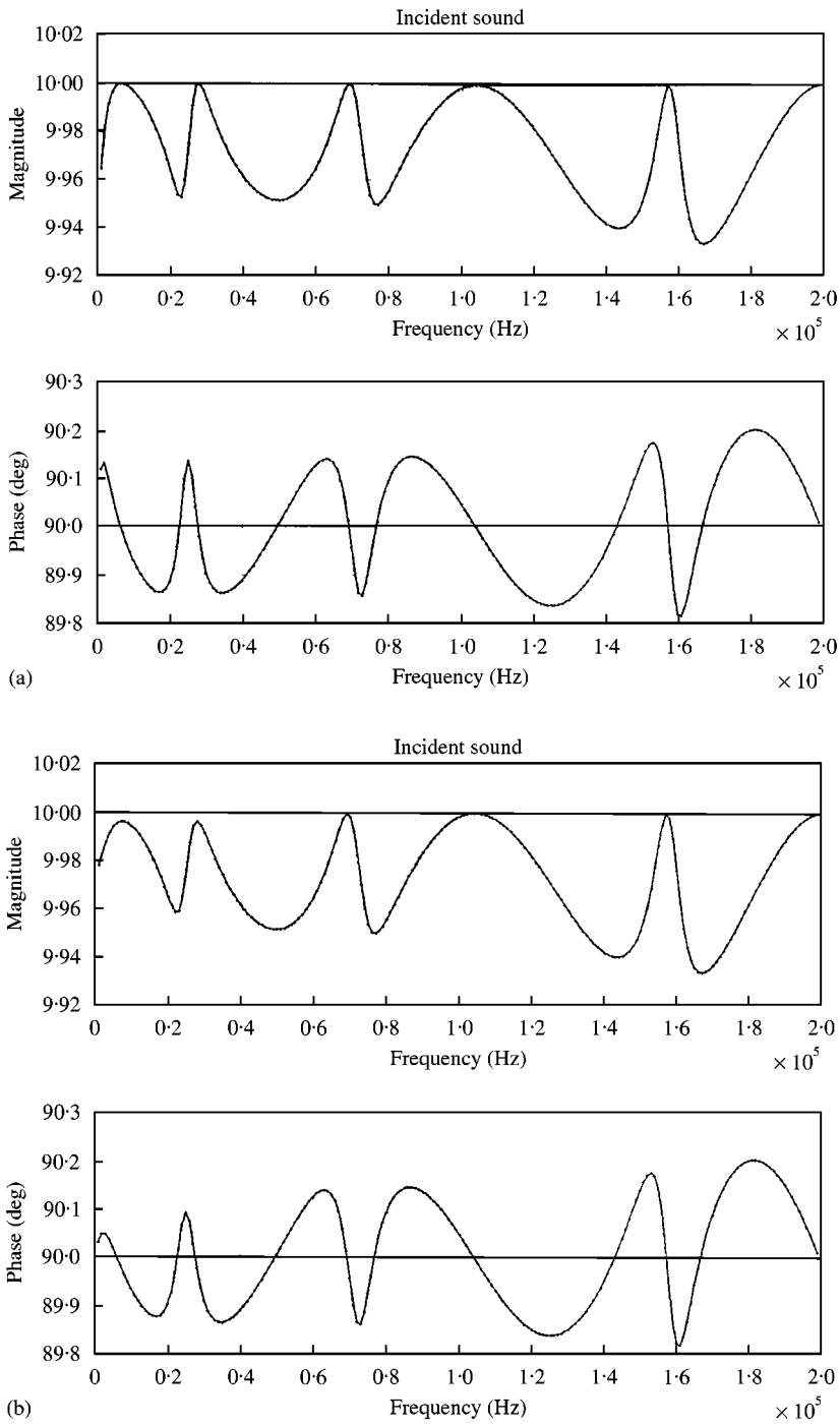
Figure 12. The comparison of calculated and actual incident sound wave: (a) upper medium is water and lower is air and (b) upper medium is water and lower is water. —, given p^{in} ; ----, calculated p^{in} from two sensors.
