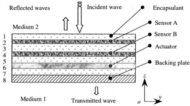
Figure 10. A backing plate covered by a coating with integrated sensors and an actuator.
